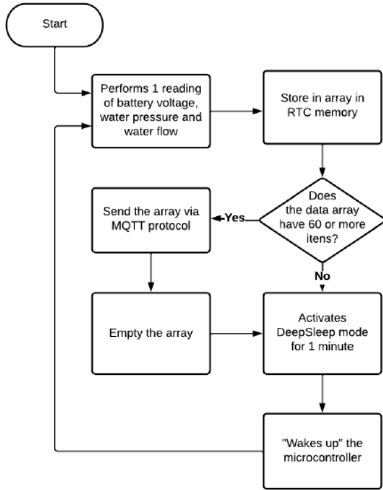
Fig. 8. Operation Logic.
