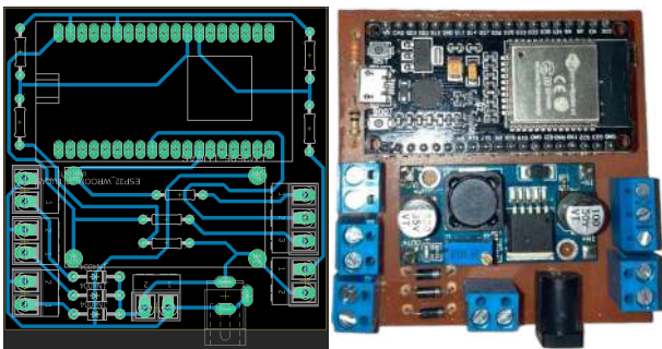
Fig. 6. Developed Hardware.
