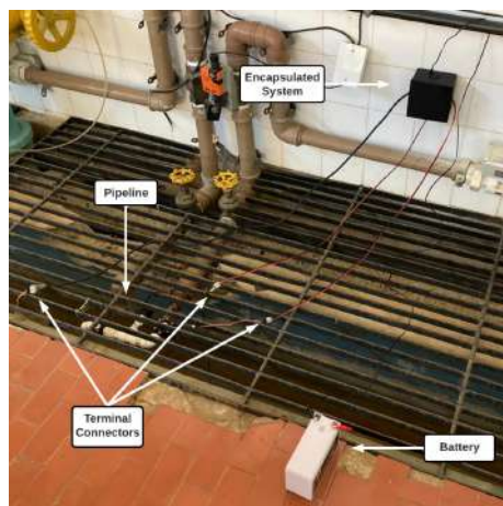
Fig. 10. System operating.
