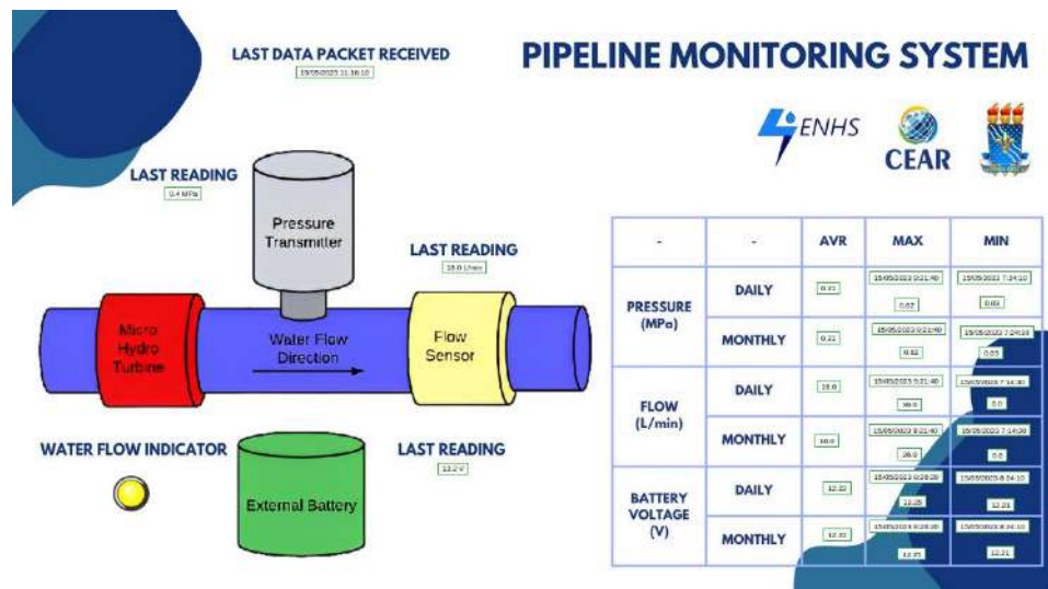
Fig. 9. Monitoring System.
