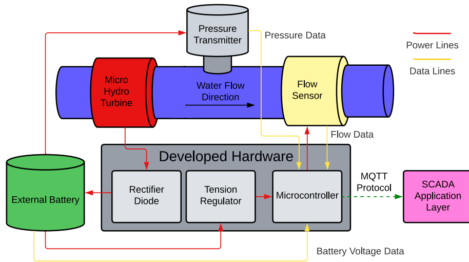
Fig. 1. System Schematic.
